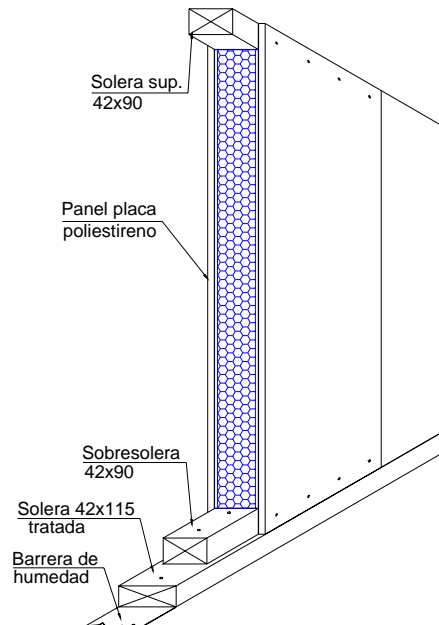
Fig. 1 Detalle panel
